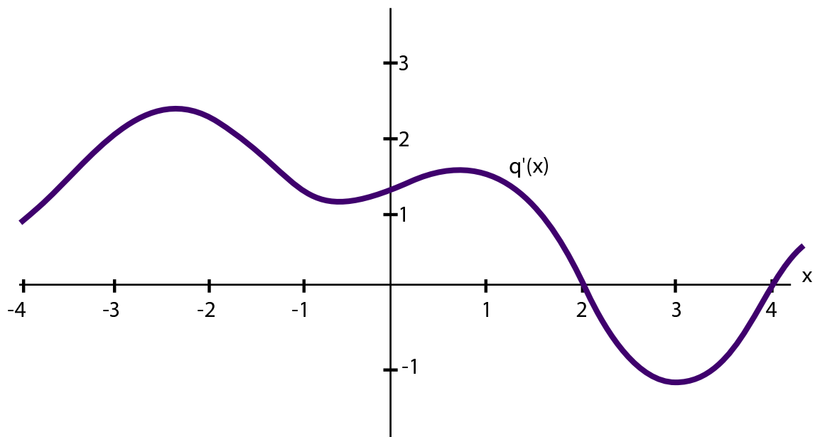
Figure 1: NOT the graph of q(x)
